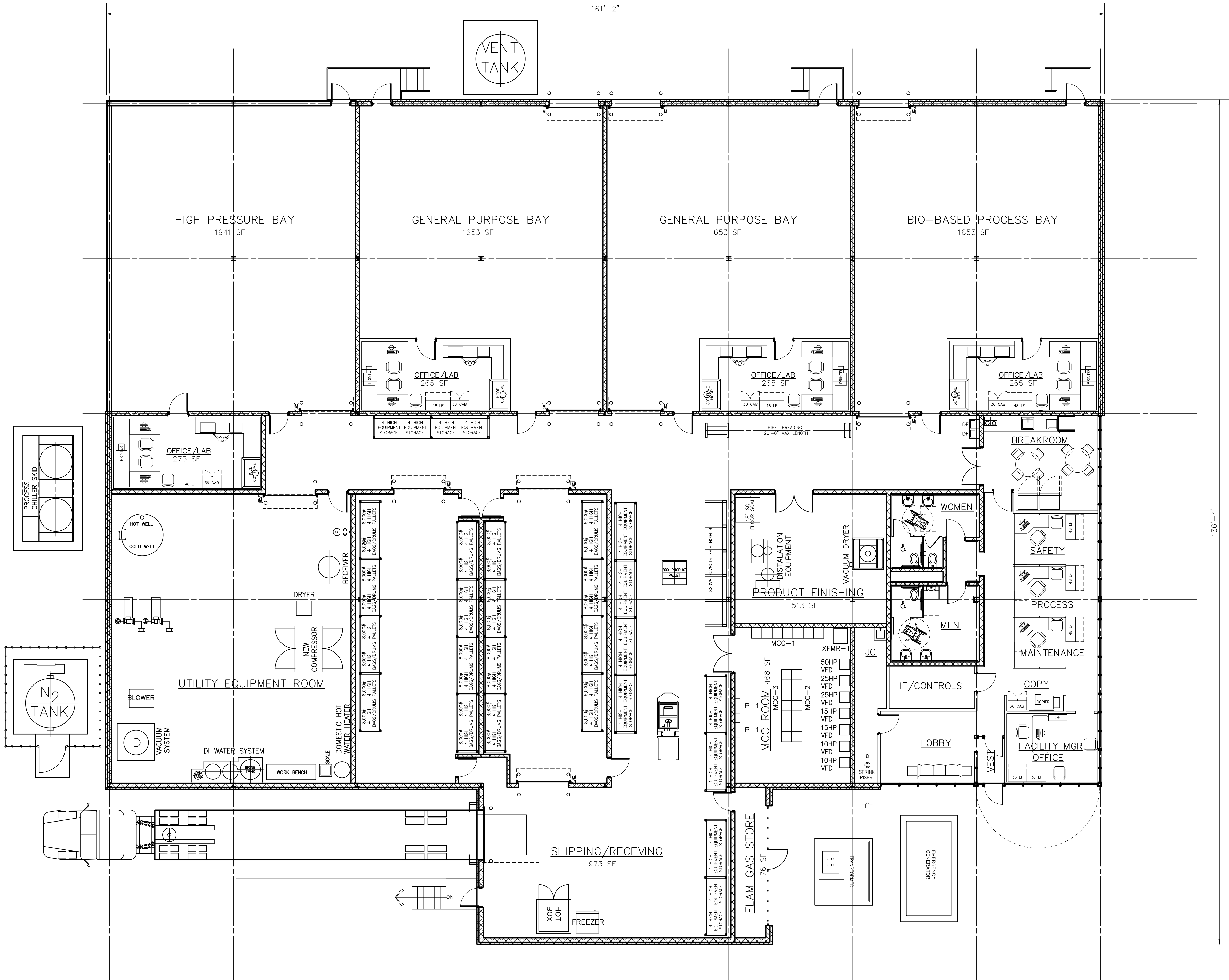
PROPOSED PILOT PLANT FACILITY 18,922 SF GROSS
